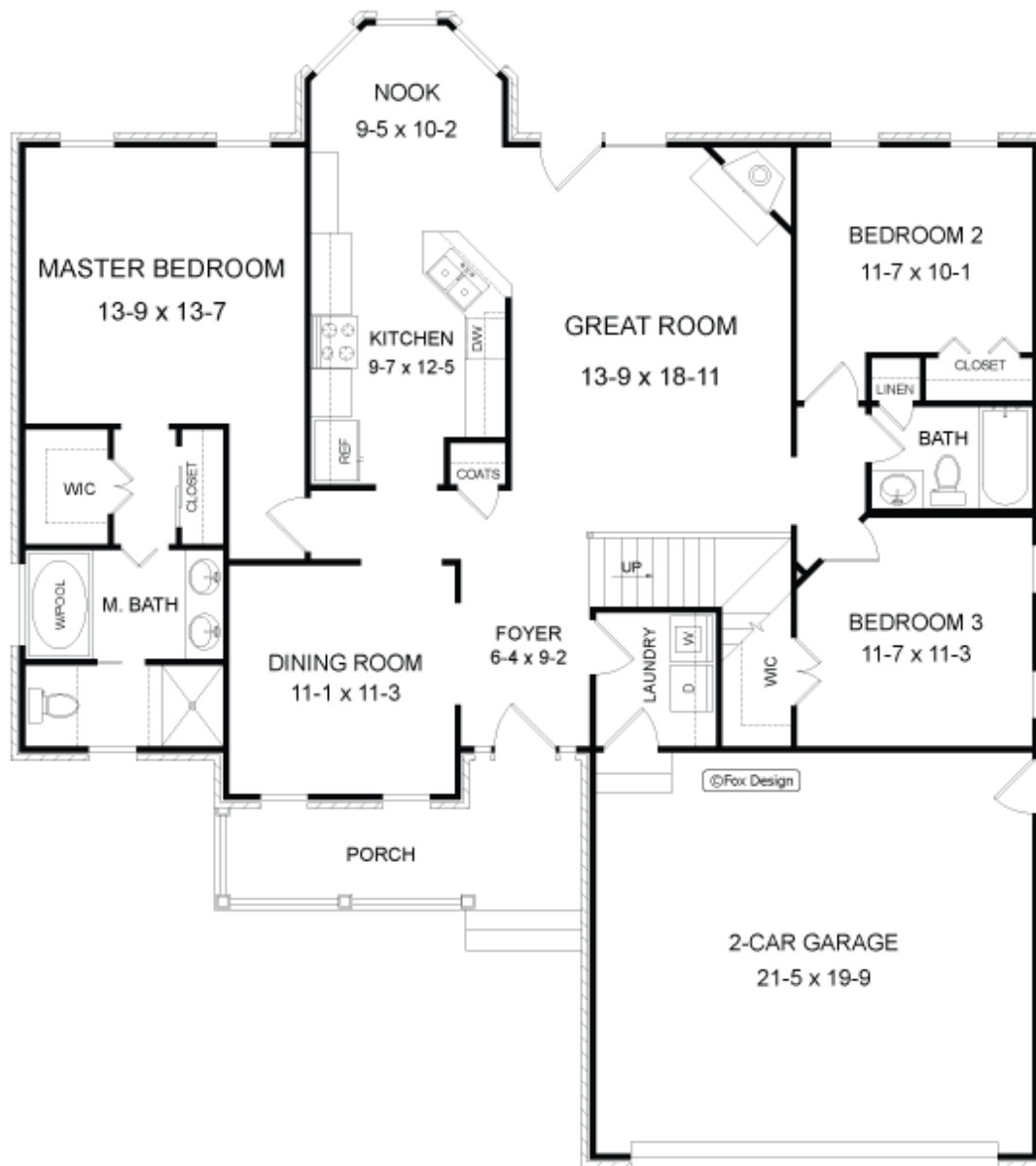
FIRST FLOOR
